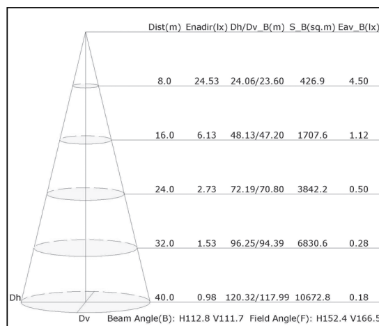
CURVE LUX/DISTANZA
